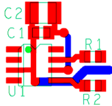
Figure 24. External Component Placement Example
