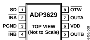
Figure 7. ADP3629 Pin Configuration
