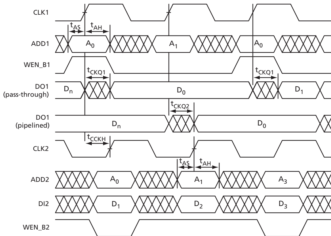
Figure 2-56 • Write Access After Read onto Same Address
