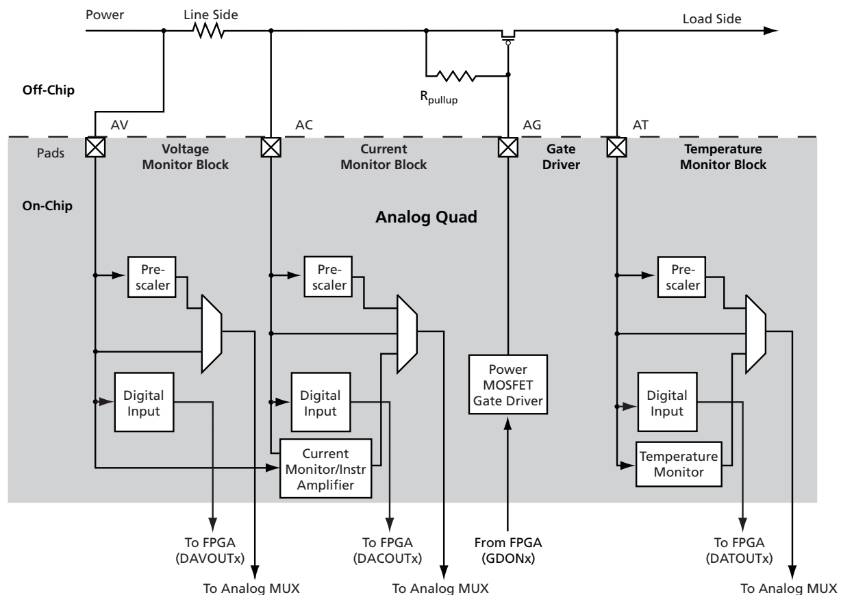
Figure 1-1 • Analog Quad
