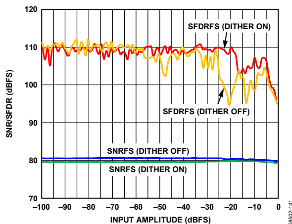
Figure 41. AD9265-125 Single-Tone SNR/SFDR vs. Input Amplitude ( A_{IN} ) with f_{IN} = 30 MHz With and Without Dither Enabled
