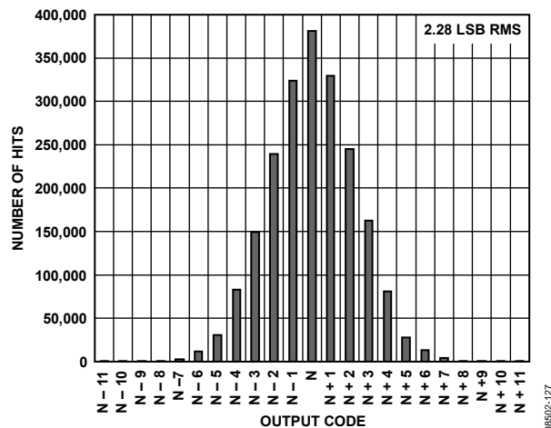
Figure 27. AD9265-105 Grounded Input Histogram
