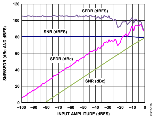
Figure 39. AD9265-125 Single-Tone SNR/SFDR vs. Input Amplitude ( A_{IN} ) with f_{IN} = 2.4 MHz
