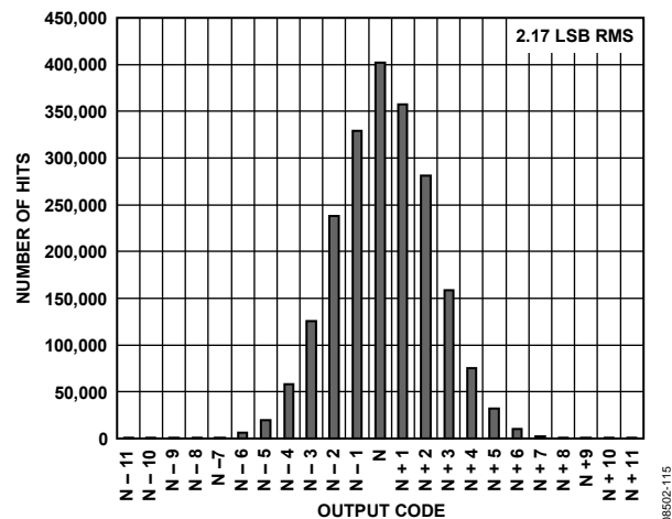
Figure 15. AD9265-80 Grounded Input Histogram
