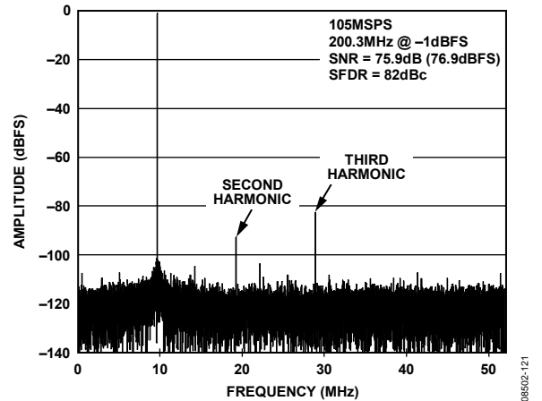
Figure 21. AD9265-105 Single-Tone FFT with f_{IN} = 200.3 MHz
