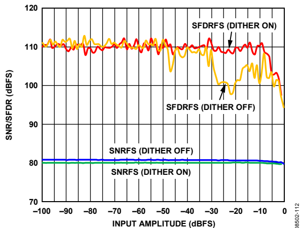
Figure 12. AD9265-80 Single-Tone SNR/SFDR vs. Input Amplitude ( A_{IN} ) with f_{IN} = 30 MHz With and Without Dither Enabled
