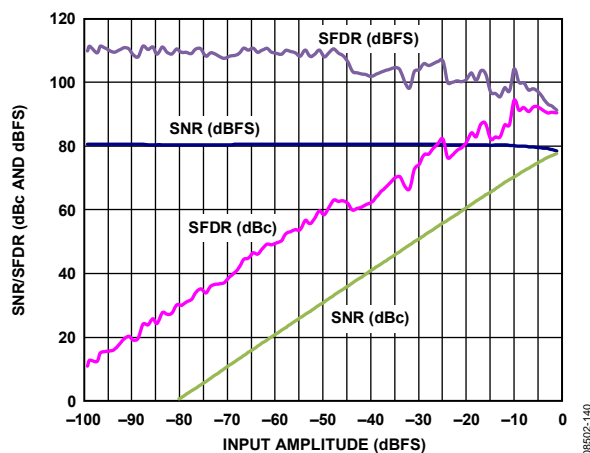
Figure 40. AD9265-125 Single-Tone SNR/SFDR vs. Input Amplitude ( A_{IN} ) with f_{IN} = 98.12 MHz
