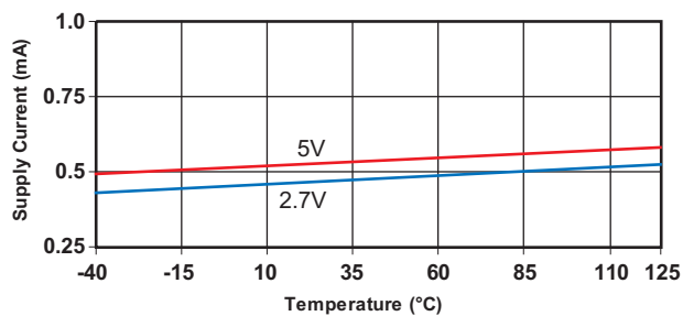
Figure 6. Supply Current vs. Temperature
