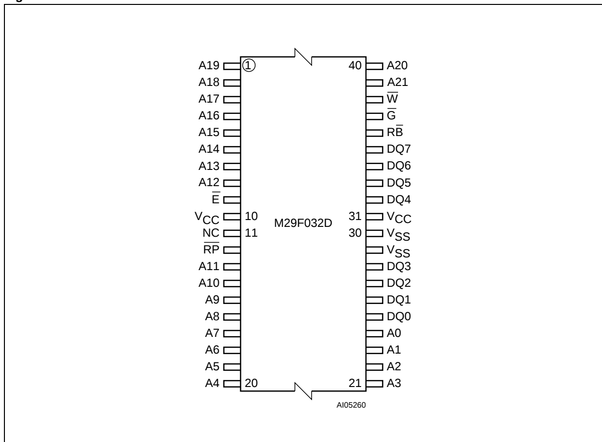
Figure 3. TSOP Connections
