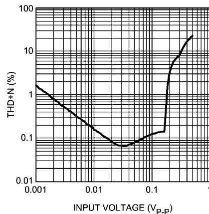
THD+N vs Input Voltage f = 1\text{kHz} Mic2 Pass Through Mode
