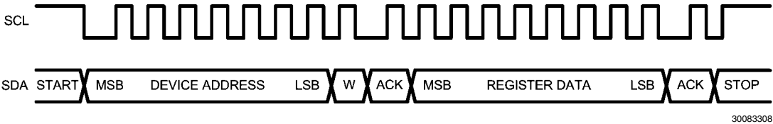
FIGURE 7. Start and Stop Diagram
