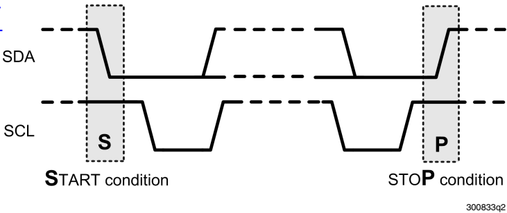
FIGURE 6. I 2 C Start Stop Conditions
