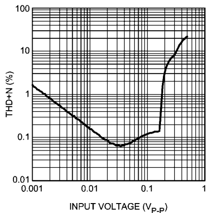
THD+N vs Input Voltage 查询"LMV1090"供应商 Mic1 Pass Through Mode
