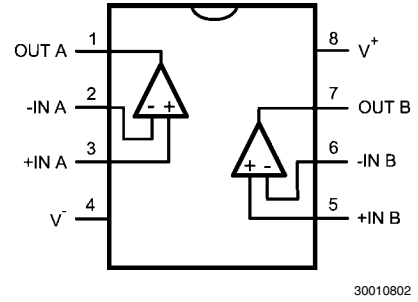
8-Pin SOIC/MSOP (LMP7718)
