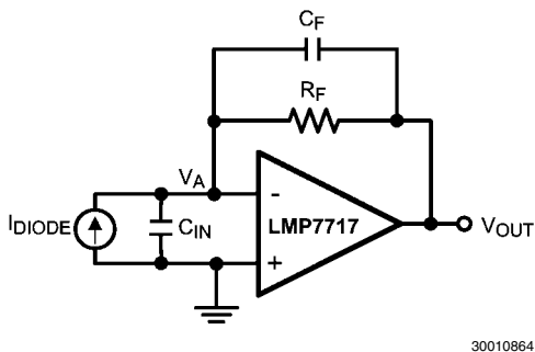
FIGURE 17. Transimpedance Feedback Model
