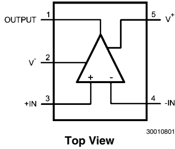
5-Pin SOT-23 (LMP7717)
