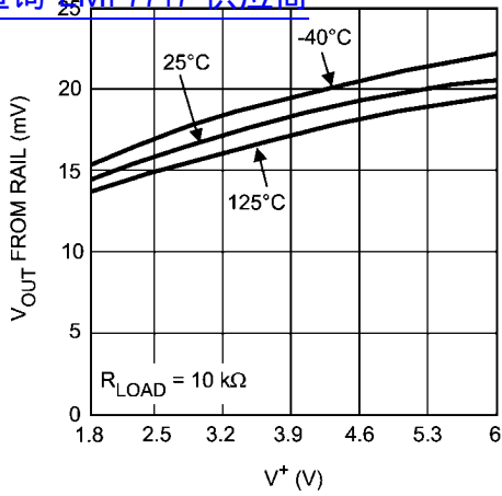
Negative Output Swing vs. Supply Voltage 查询"LMP7717"供应商
