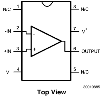
8-Pin SOIC (LMP7717)
