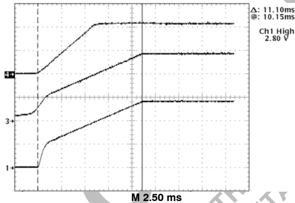
Figure 4. CS5157 Demonstration Board Startup in Response to Increasing 12 V and 5.0 V Input Voltages. Extended Off Time is Followed by Normal Off Time Operation when Output Voltage Achieves Regulation to the Error Amplifier Output.
