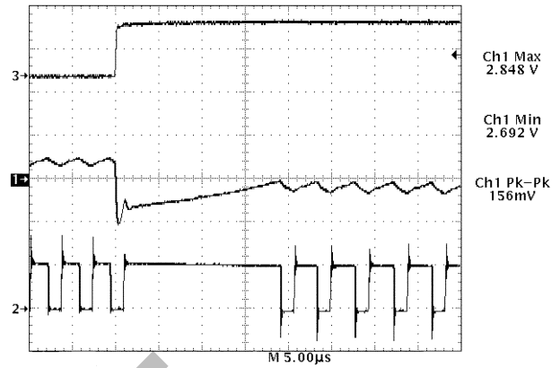
Figure 10. CS5157 Demonstration Board Response to 13 A Load Turn On (Output Set for 2.8 V). Upon Completing a Normal Off Time, The V^2 Control Loop Immediately Connects the Inductor to the Input Voltage, Providing 100% Duty Cycle. Regulation is Achieved in Less Than 20 \mu s
