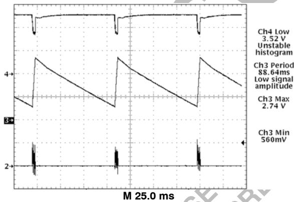
Figure 12. CS5157 Demonstration Board Hiccup Mode Short Circuit Protection. Gate Pulses are Delivered While the Soft Start Capacitor Charges, and Cease During Discharge
