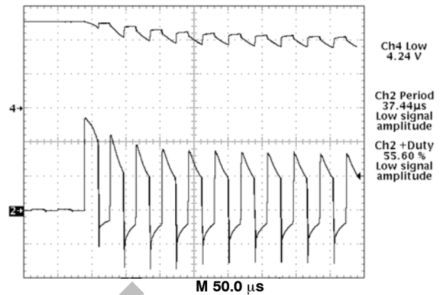
Figure 13. Startup with Regulator Output Shorted
