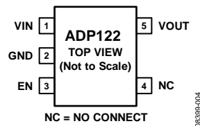
Figure 3. ADP122 Fixed Output Pin Configuration
