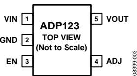
Figure 4. ADP123 Adjustable Output Pin Configuration
