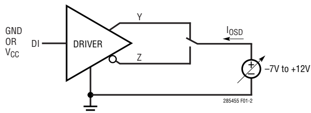
Figure 2. Driver Output Short-Circuit Current
