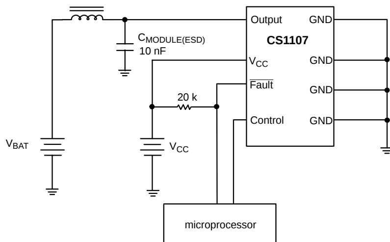
Figure 2. Applications Diagram
