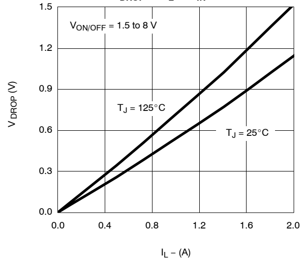
V_{DROP} vs. I_L @ V_{IN} = 1.8 V
