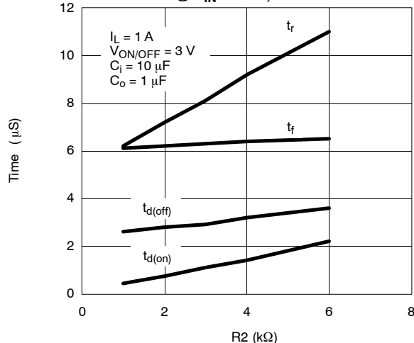
Switching Variation R2 @ V_{IN} = 1.8 V , R1 = 20 k \Omega
