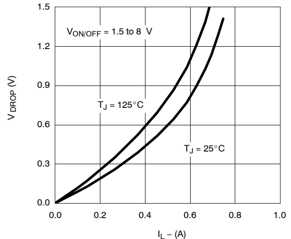
V_{DROP} vs. I_L @ V_{IN} = 1.8 V
