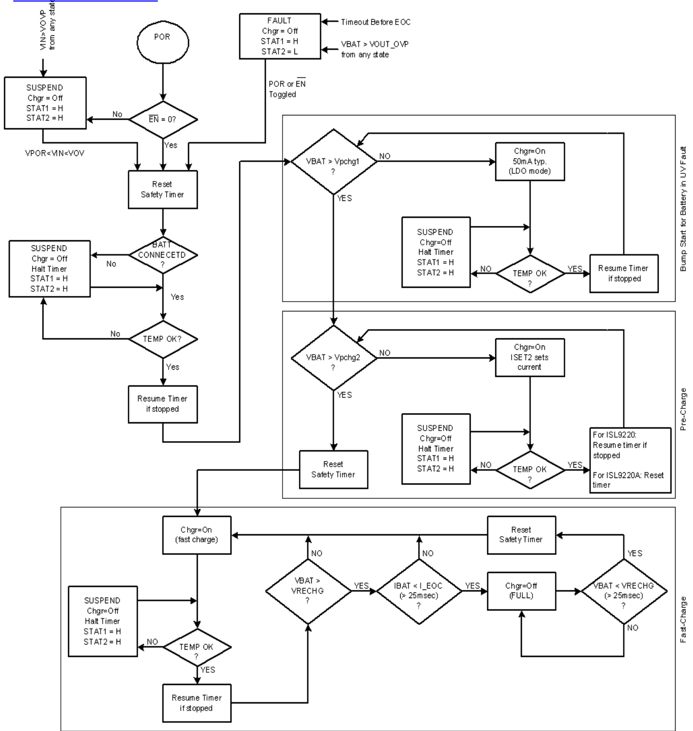
FIGURE 9. CHARGING FLOW CHART
