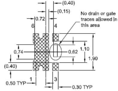
RECOMMENDED LAND PATTERN OPT 1
