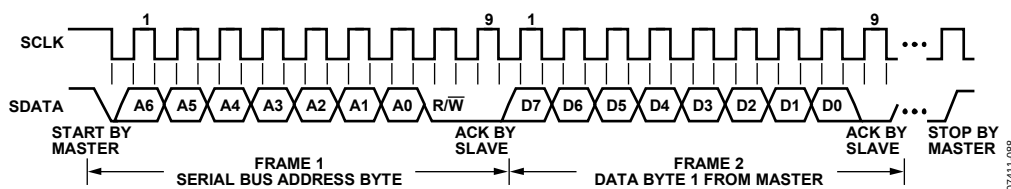
Figure 115. I 2 C Write Operation
