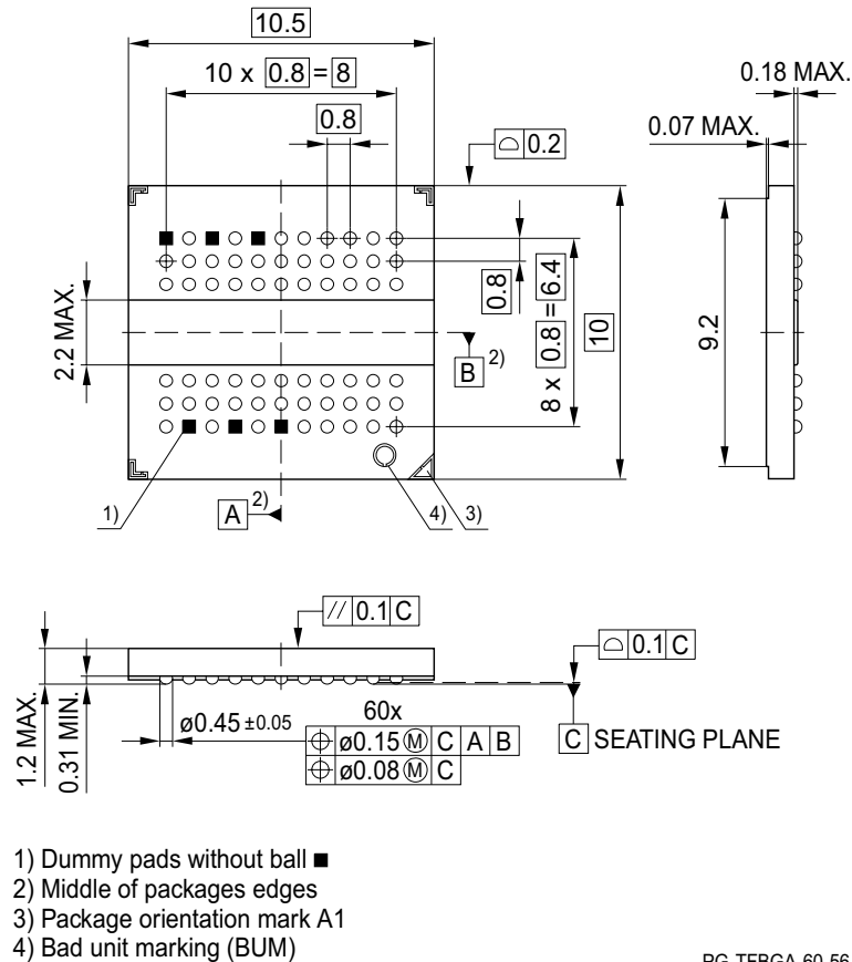
FIGURE 9 Package Outline PG-TFBGA-60
