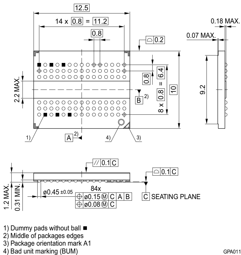
FIGURE 8 Package Outline PG-TFBGA-84
