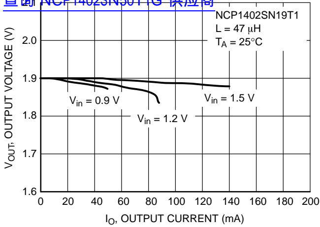
Figure 3. NCP1402SN19T1 Output Voltage vs. Output Current
