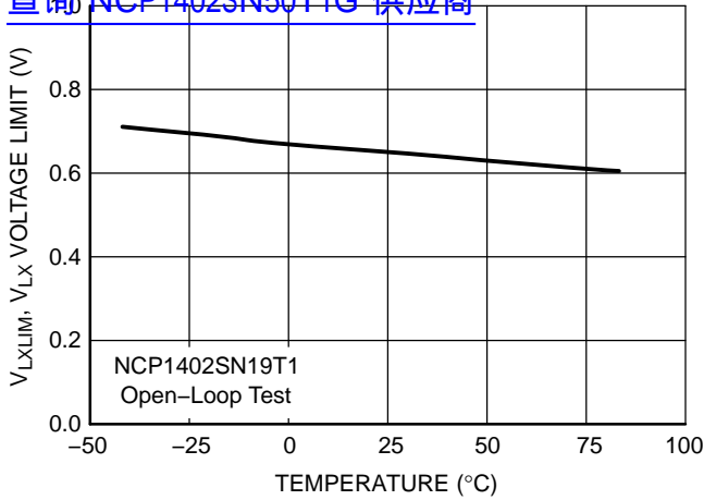
Figure 27. NCP1402SN19T1 V_{LX} Voltage Limit vs. Temperature
