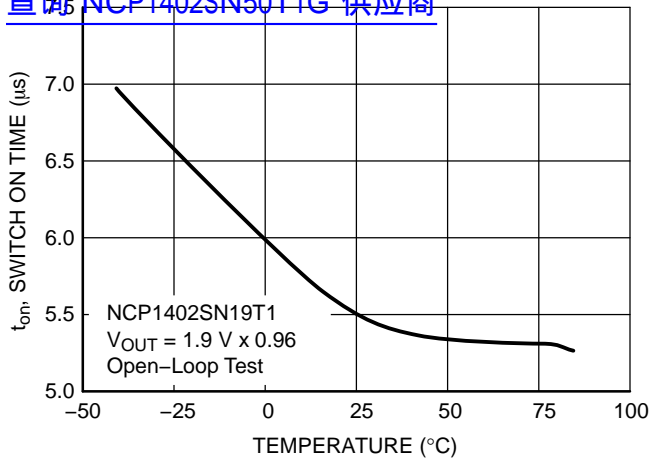
Figure 15. NCP1402SN19T1 Switch On Time vs. Temperature
