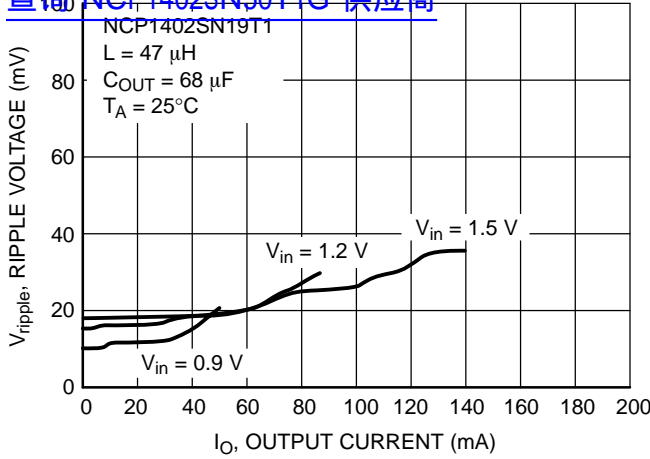
Figure 51. NCP1402SN19T1 Ripple Voltage vs. Output Current
