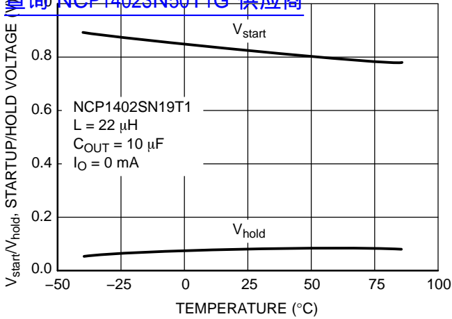
Figure 33. NCP1402SN19T1 Startup/Hold Voltage vs. Temperature
