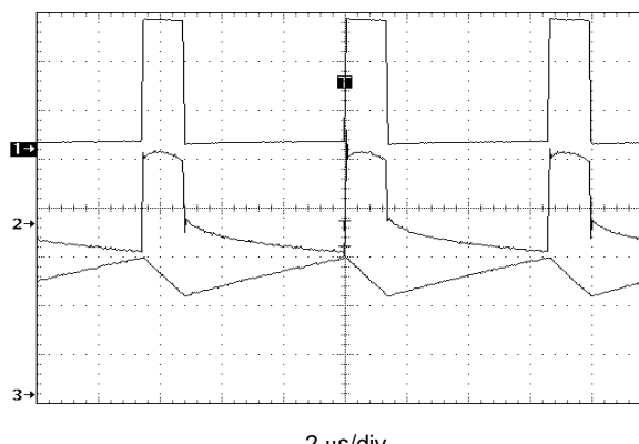
Figure 42. NCP1402SN30T1 Operating Waveforms (Heavy Load)
