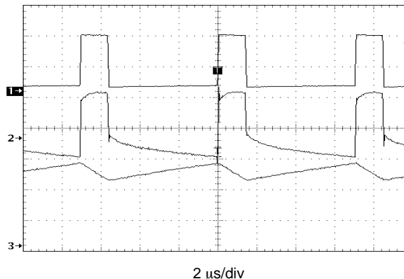
Figure 40. NCP1402SN19T1 Operating Waveforms (Heavy Load)
