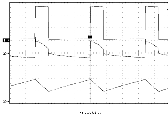
Figure 41. NCP1402SN30T1 Operating Waveforms (Medium Load)
