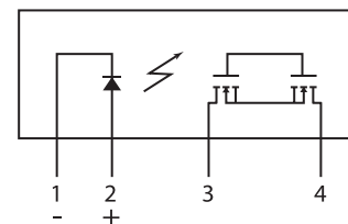
CPC1906Y Pinout
