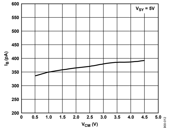
Figure 17. Input Bias Current vs. Input Common-Mode Voltage at 125°C
