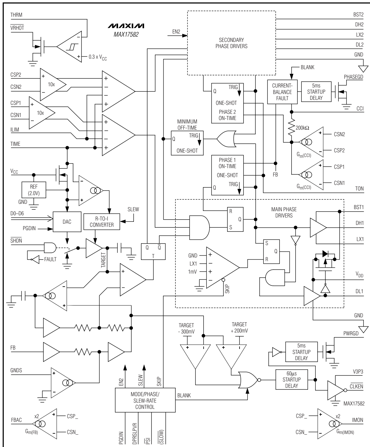
Figure 2. Functional Diagram
