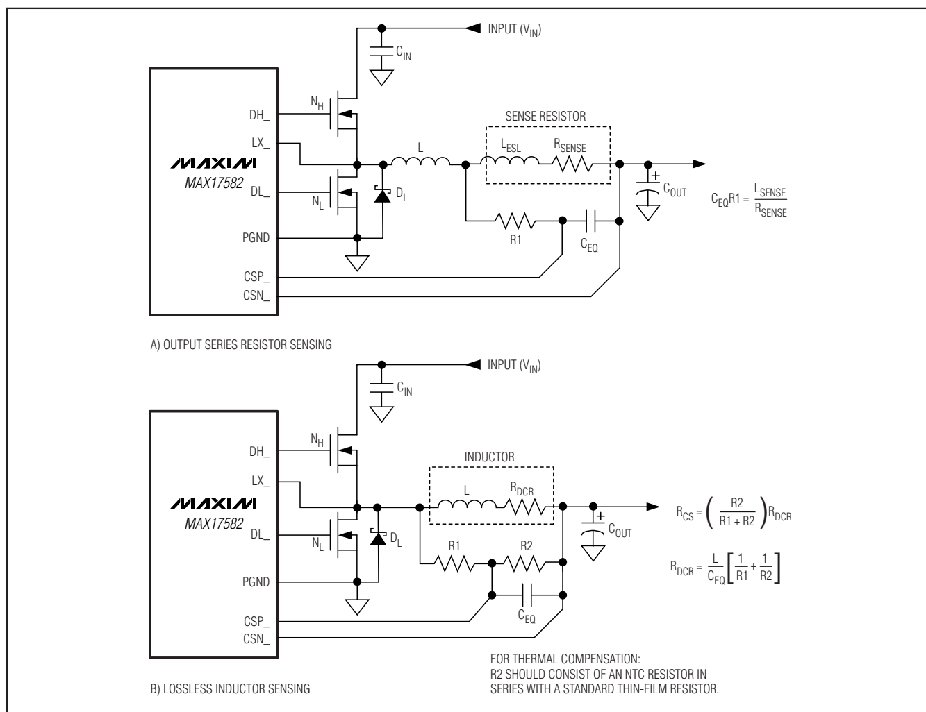
Figure 3. Current-Sense Methods
