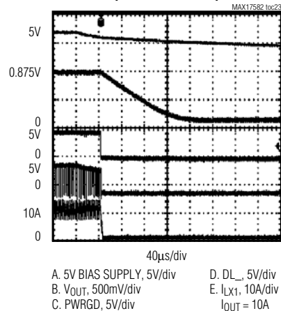
BIAS SUPPLY REMOVAL (UVLO RESPONSE)
