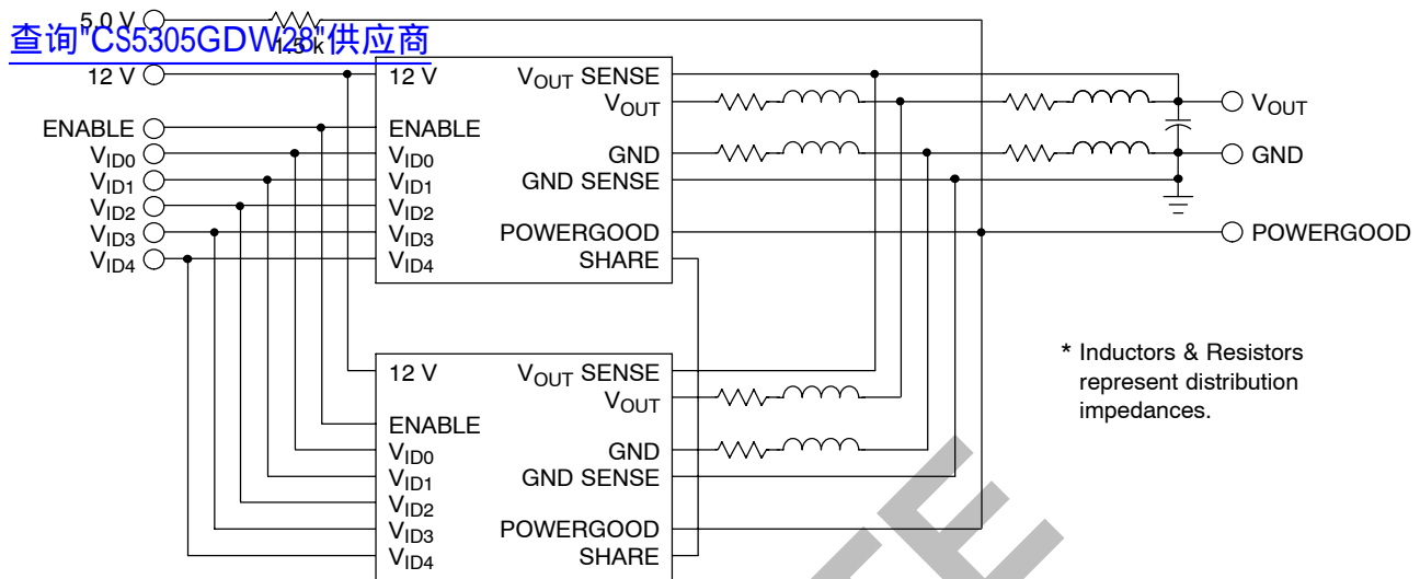
Figure 2. Two-Converter System with Sharing
