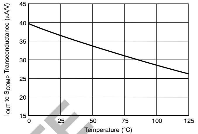
Figure 23. I_{OUT} to S_{COMP} Transconductance vs. Temperature
