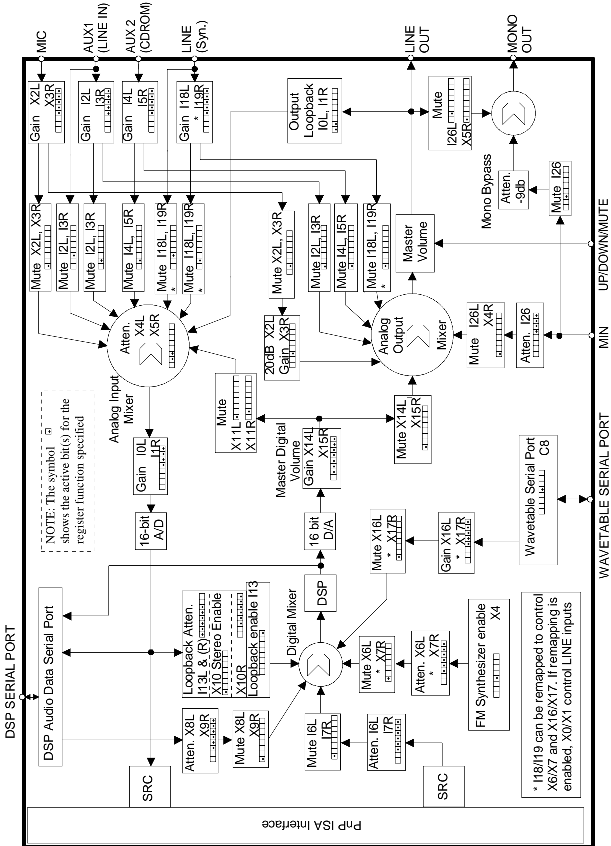
Figure 4. MODE 3 Mixer (assumes IFM or WTEN is set)
