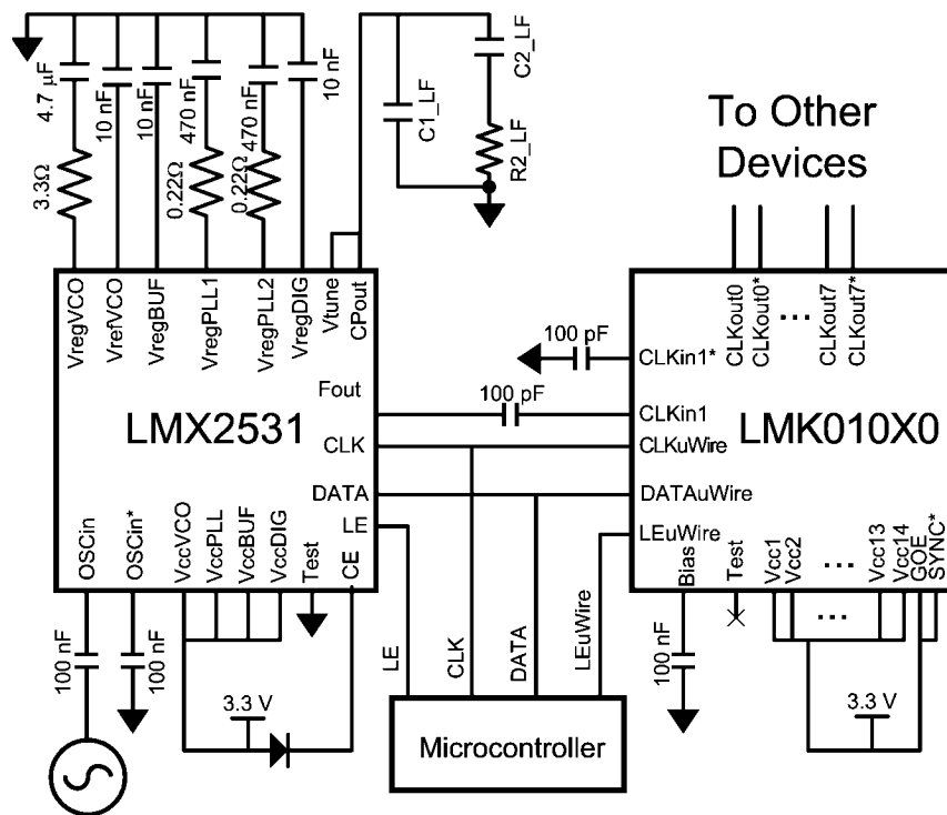
FIGURE 1. Typical Application
