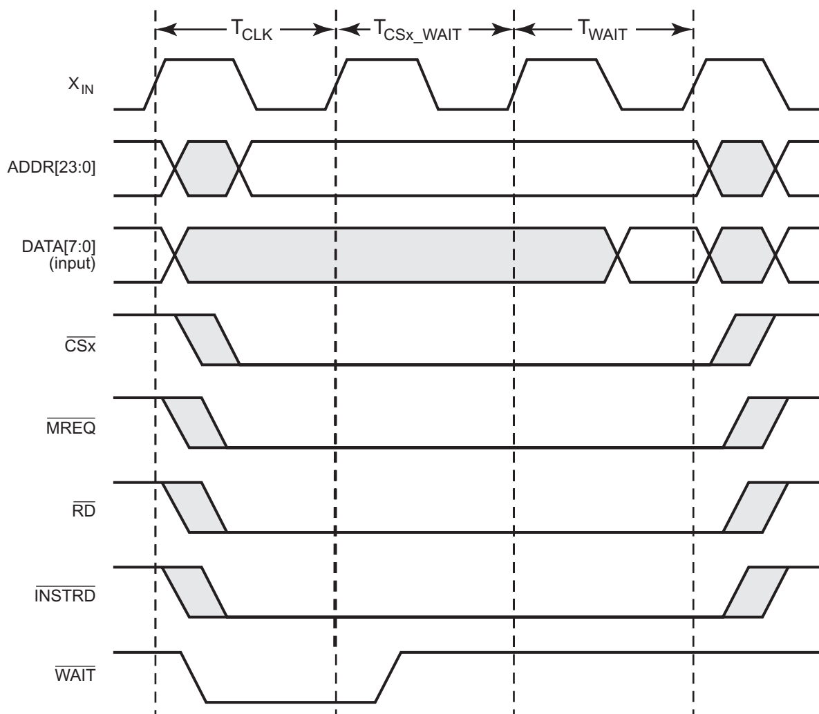
Figure 6. Wait State Operation Example (Read Operation)
