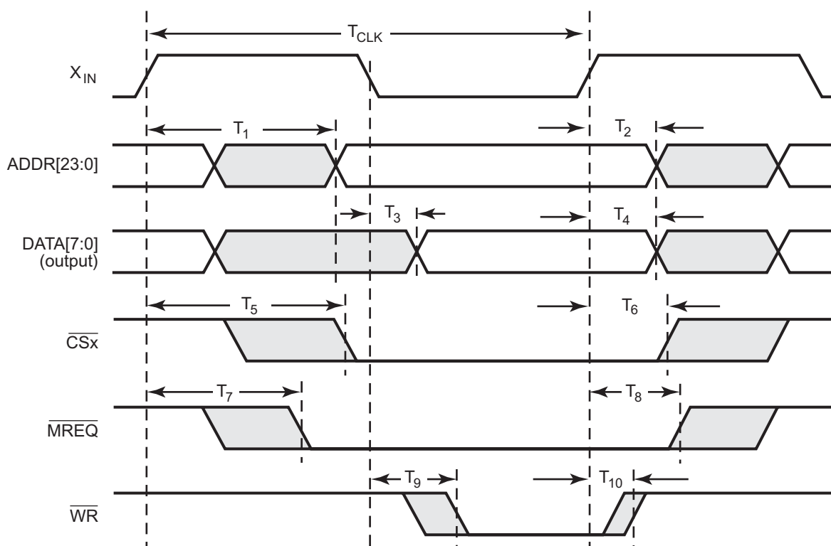
Figure 49. External Memory Write Timing
