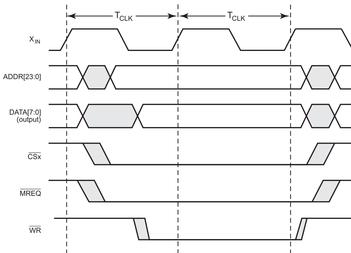
Figure 54. Wait State Timing for Write Operations
