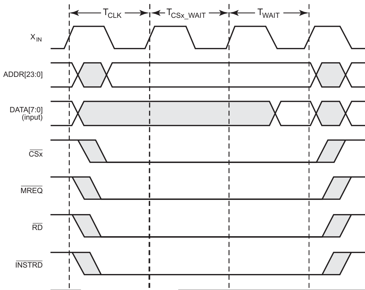
Figure 53. Wait State Timing for Read Operations
