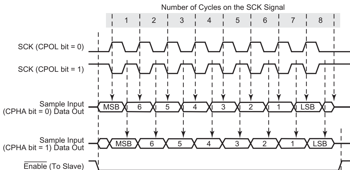
Figure 29. SPI Timing
