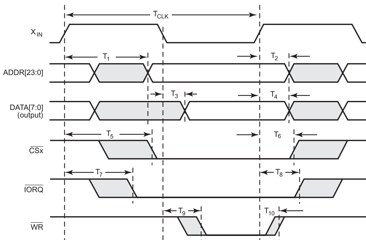
Figure 52. External I/O Write Timing
