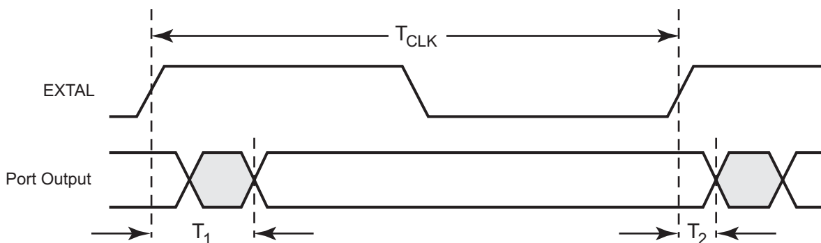
Figure 56. GPIO Port Output Timing
