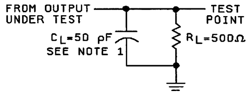
LOAD CIRCUIT FOR TOTEM-POLE OUTPUTS
