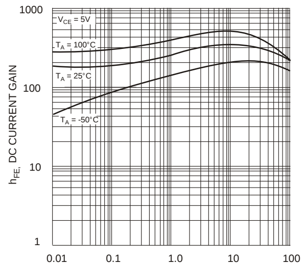
Fig. 2, DC Current Gain vs. Collector Current (BC847B)
