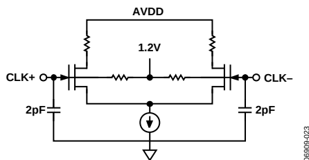
Figure 55. Equivalent Clock Input Circuit
