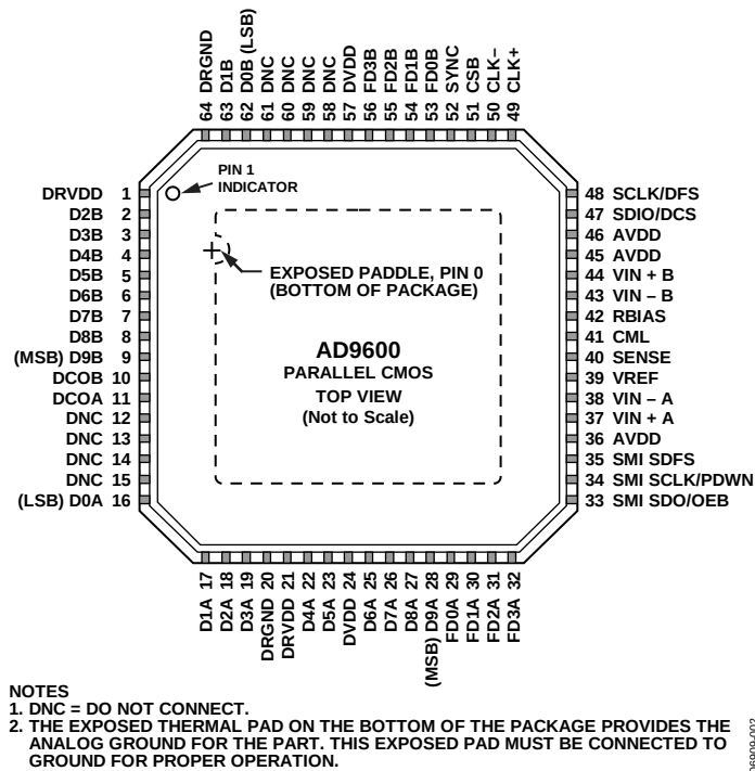
Figure 6. Parallel CMOS Mode Pin Configuration (Top View)
