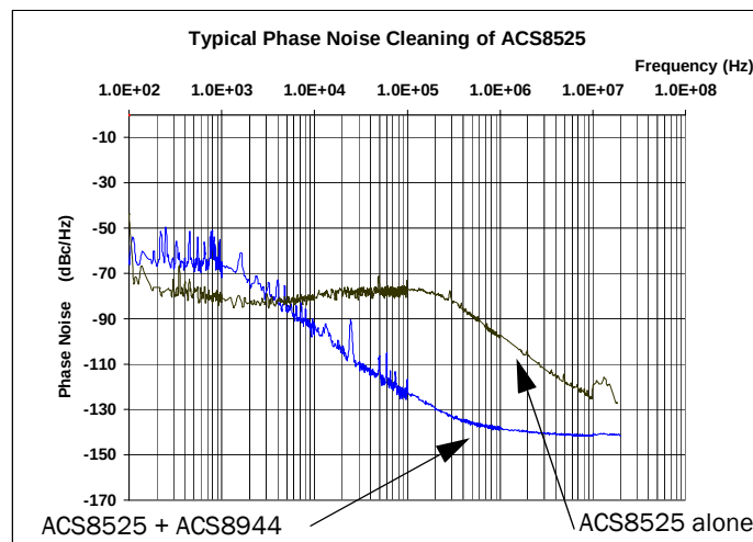
Figure 7 Phase Offset from Carrier, ACS8525 with/without ACS8944
