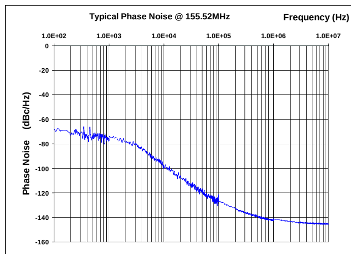
Figure 6 Phase Offset from Carrier, ACS8944
