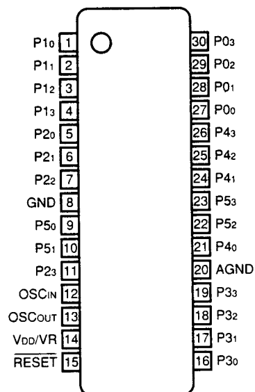
30-PIN SDIP
