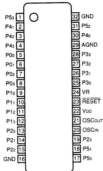
32-PIN SOP
