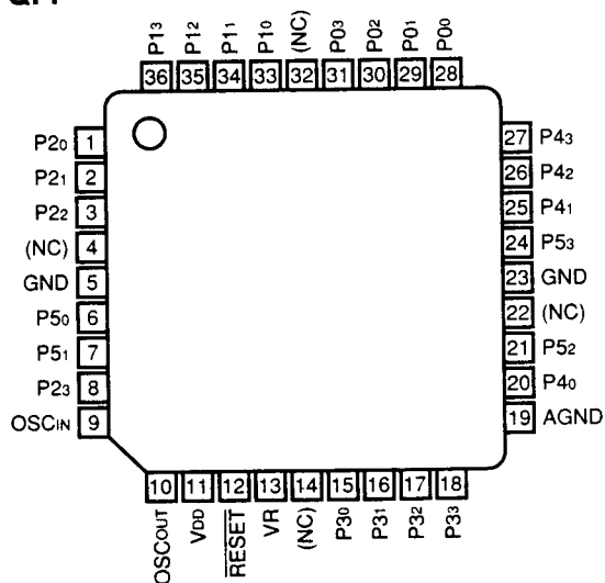
36-PIN QFP
