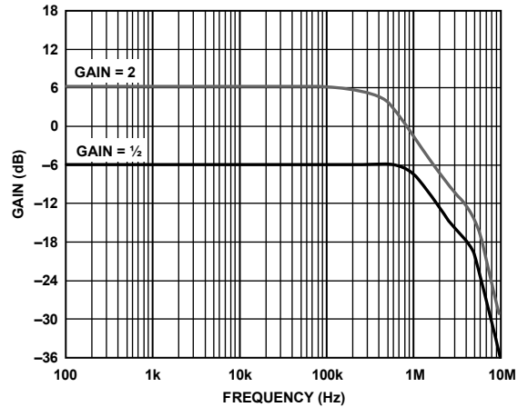
Figure 16. Gain vs. Frequency, \pm 15V Supplies
