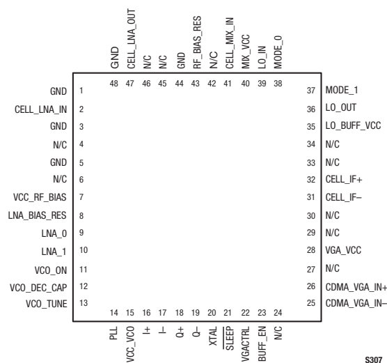
Figure 1. SKY74691 Pinout – 48-Pin RFLGA (Top View)
