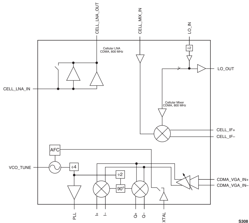
Figure 2. SKY74691 Receiver Block Diagram
