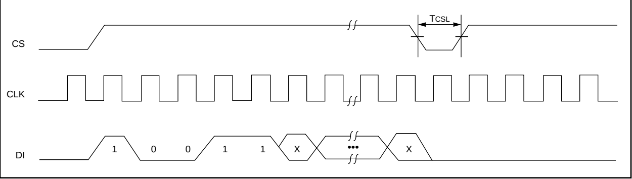
FIGURE 3-5: EWEN TIMING
