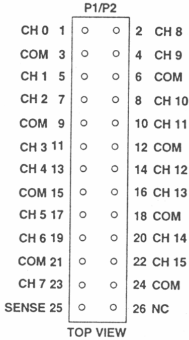
Figure 3 5B01 Pin-outs
