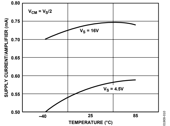
Figure 10. Supply Current/Amplifier vs. Temperature
