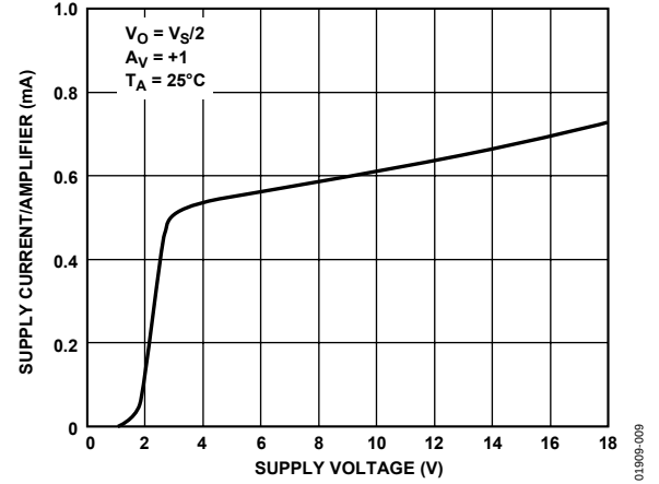
Figure 9. Supply Current/Amplifier vs. Supply Voltage
