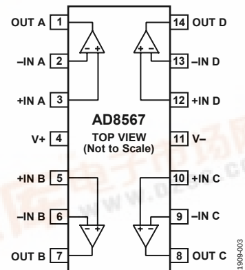
Figure 3. 14-Lead TSSOP Pin Configuration
