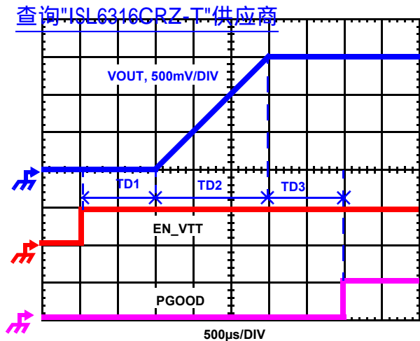
FIGURE 11. SOFT-START WAVEFORMS
