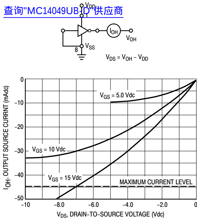
Figure 5. Typical Output Source Characteristics
