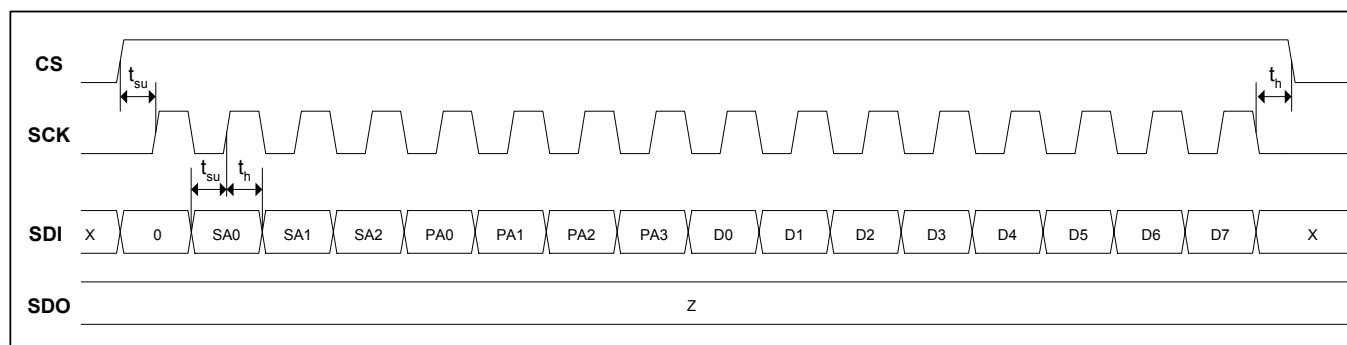
Figure 10: Write Operation
