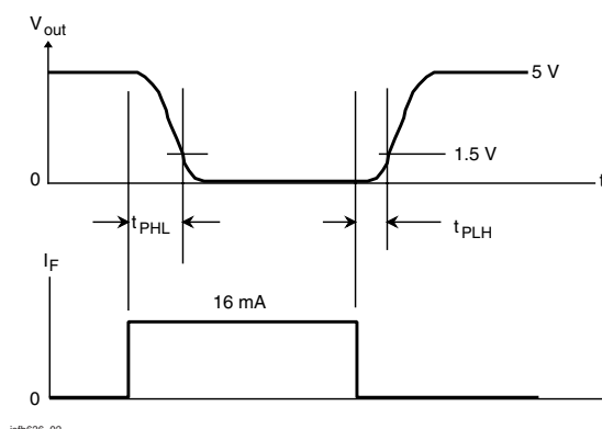
Fig. 2 - Switching Time Measurement
