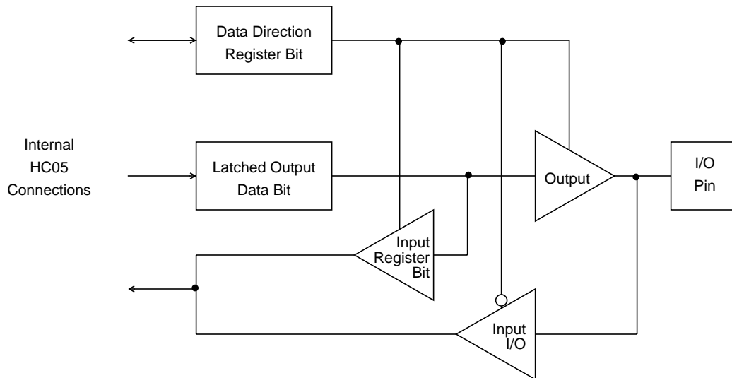
Figure 3-3. Port I/O Circuitry
