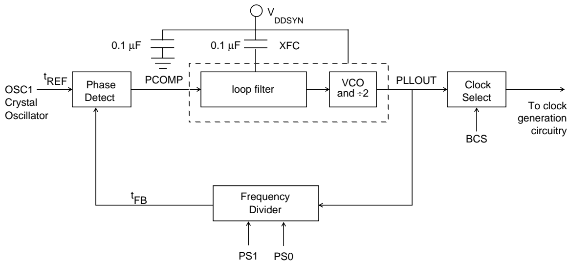
Figure 6-4. PLL Circuit
