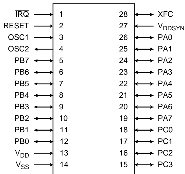
Figure 2-1. Single-Chip Mode Pinout of the MC68HC05E1
