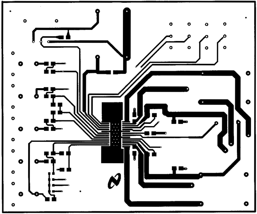
FIGURE 8. Top Layer - ( Not to Scale )
