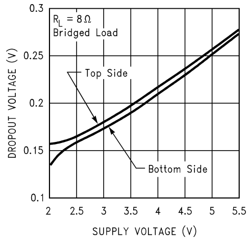
Dropout Voltage
