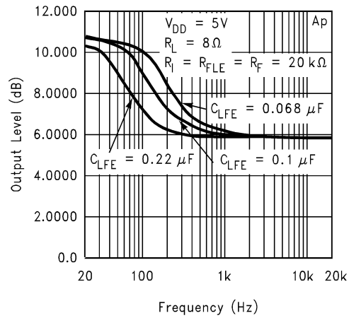
External Gain/Bass Boost Characteristics
