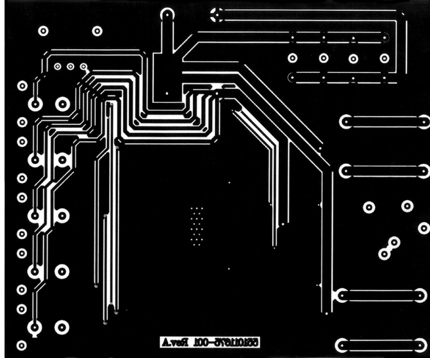
FIGURE 9. Bottom Layer - ( Not to Scale )
