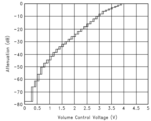
Volume Control Characteristics
