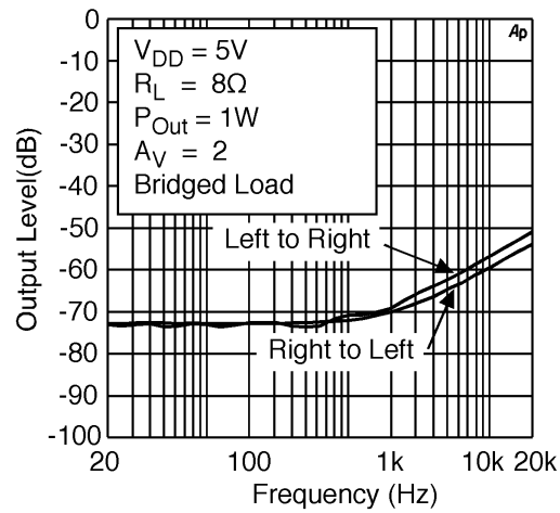
Crosstalk
