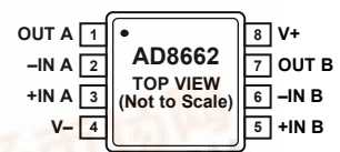
Figure 4. AD8662, 8-Lead MSOP (RM-8)
