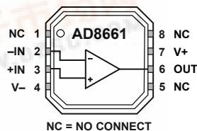
Figure 2. AD8661, 8-Lead LFCSP_VD (CP-8-2)
