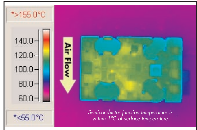
Figure 10: Thermal plot of converter at 15A load on 2.5V output and 11.5A load on 3.3V output with 70°C air flowing at 200 LFM. Air flow across the converter is from pin 1 to pin 3 (nominal input voltage).
