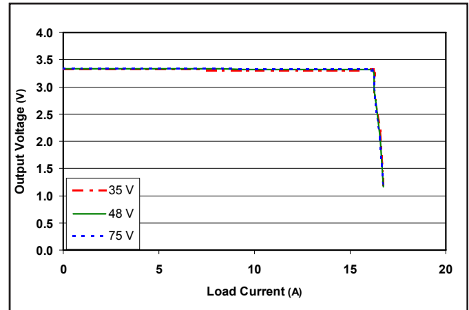
Figure 22: Output voltage vs. load current showing typical current limit curves and converter shutdown points for the 3.3V output. 2.5V load is at 0A.
