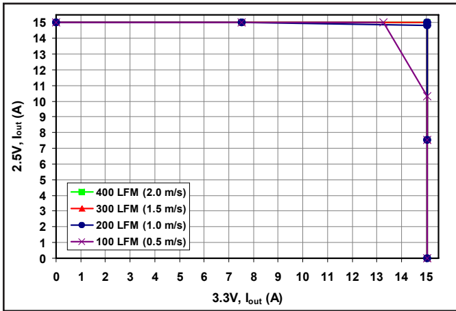
Figure 7: Maximum output power derating curves at 55°C vs. airflow rates of 100 through 400 LFM. Curve shows available current for 2.5V rail on y axis and available current for 3.3V rail on x axis. (nom. V_{in} )
