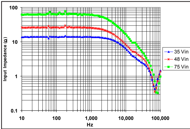
Figure 31: Input impedance ( Z_{in} = V_{in}/I_{in} ) for minimum, nominal, and maximum input voltage at full rated power for 2.5V output.
