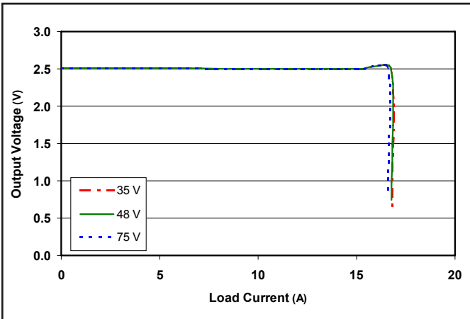
Figure 21: Output voltage vs. load current showing typical current limit curves and converter shutdown points for the 2.5V output. 3.3V load is at 0A.
