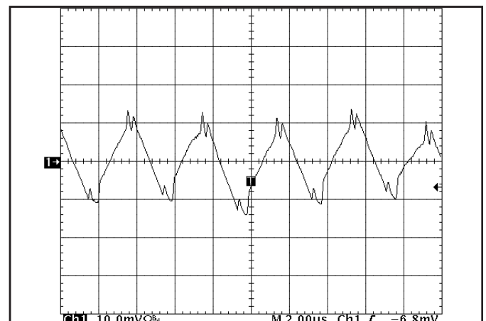
Figure 18: Input Terminal Ripple Current, 2.5V & 3.3V outputs at full rated output current and nominal input voltage with 10μH source impedance and 100μF electrolytic capacitor (10 mA/div). (see Fig. 17)
