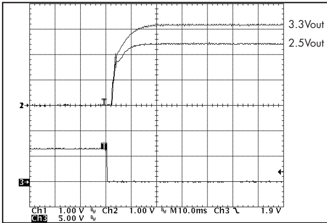
Figure 13: Turn-on transient at full rated load current (resistive load) (10 ms/div). Ch 1: 2.5Vout (1V/div); Ch 2: 3.3Vout (1V/div) Ch 3: ON/OFF input (5V/div)
