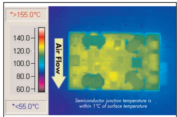
Figure 12: Thermal plot of converter at 13A load on 2.5V output and 10A load on 3.3V output with 85°C air flowing at 200 LFM. Air flow across the converter is from pin 1 to pin 3 (nominal input voltage).
