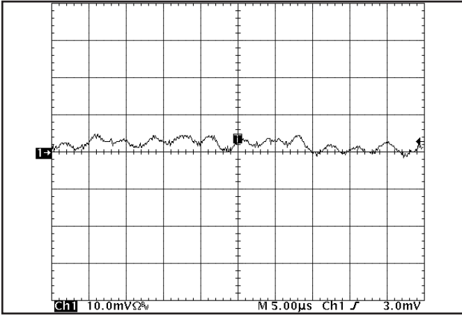
Figure 19: Input Reflected Ripple Current, i_s , through a 10 \mu H source inductor at nominal input voltage and rated load current (5 mA/div). 2.5V and 3.3V outputs at full rated load current. (see Fig. 17)
