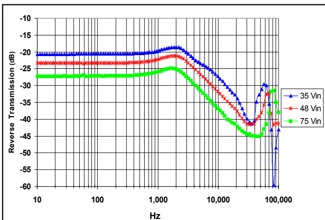
Figure 29: Reverse Transmission ( RT_1 = I_{in}/I_{out1} ) for minimum, nominal, and maximum input voltage at full rated power, for 2.5V output.
