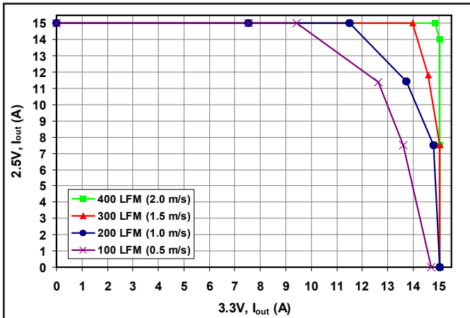
Figure 9: Maximum output power derating curves at 70°C vs. airflow rates of 100 through 400 LFM. Curve shows available current for 2.5V rail on y axis and available current for 3.3V rail on x axis. (nom. V_{in} )
