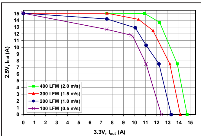
Figure 11: Maximum output power derating curves at 85°C vs. airflow rates of 100 through 400 LFM. Curve shows available current for 2.5V rail on y axis and available current for 3.3V rail on x axis. (nom. V_{in} )
