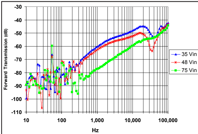
Figure 27: Forward Transmission ( FT_1 = V_{out1}/V_{in} ) for minimum, nominal, and maximum input voltage at full rated power, for 2.5V output.
