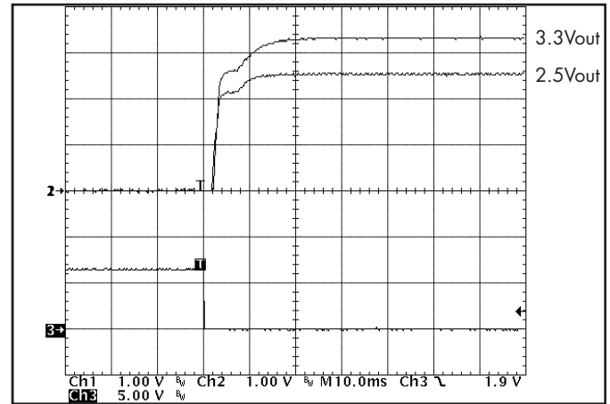
Figure 14: Turn-on transient at zero load current (10 ms/div). Ch 1: 2.5Vout (1V/div); Ch 2: 3.3Vout (1V/div) Ch 3: ON/OFF input (5V/div)
