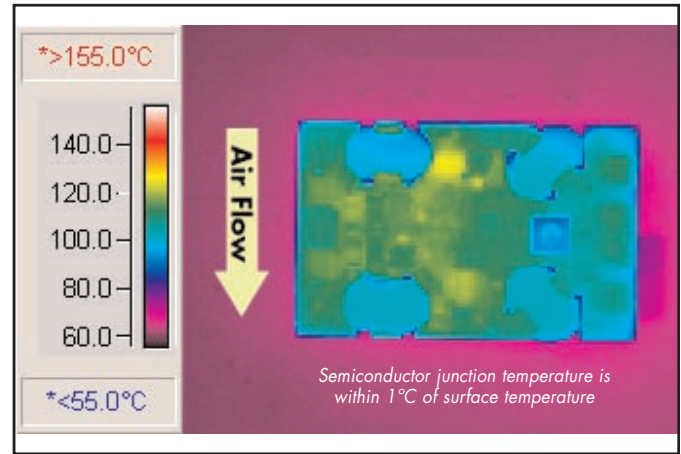
Figure 8: Thermal plot of converter at 15A load on 2.5V output and 15A load on 3.3V output with 55°C air flowing at 200 LFM. Air flow across the converter is from pin 1 to pin 3 (nominal input voltage).
