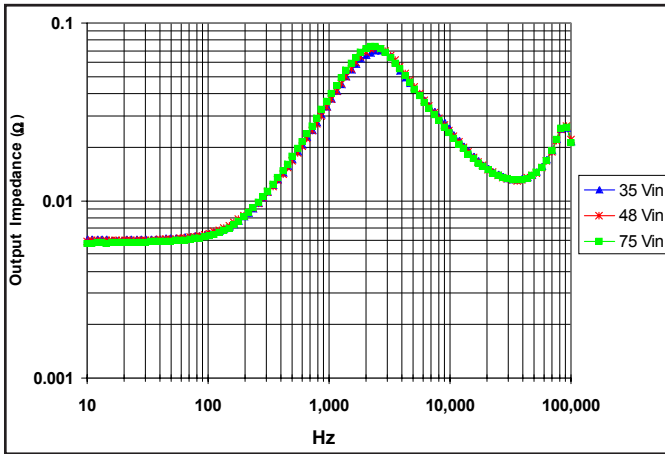
Figure 25: Output impedance ( Z_{out1} = V_{out1}/I_{out1} ) for minimum, nominal, and maximum input voltage at full rated power, for 2.5V output.
