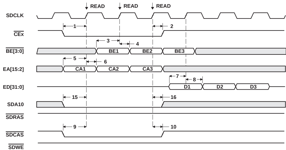
Figure 18. Three SDRAM Read Commands
