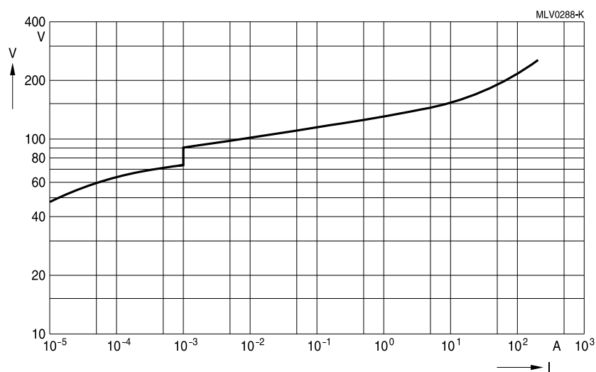
CT1210K50G
