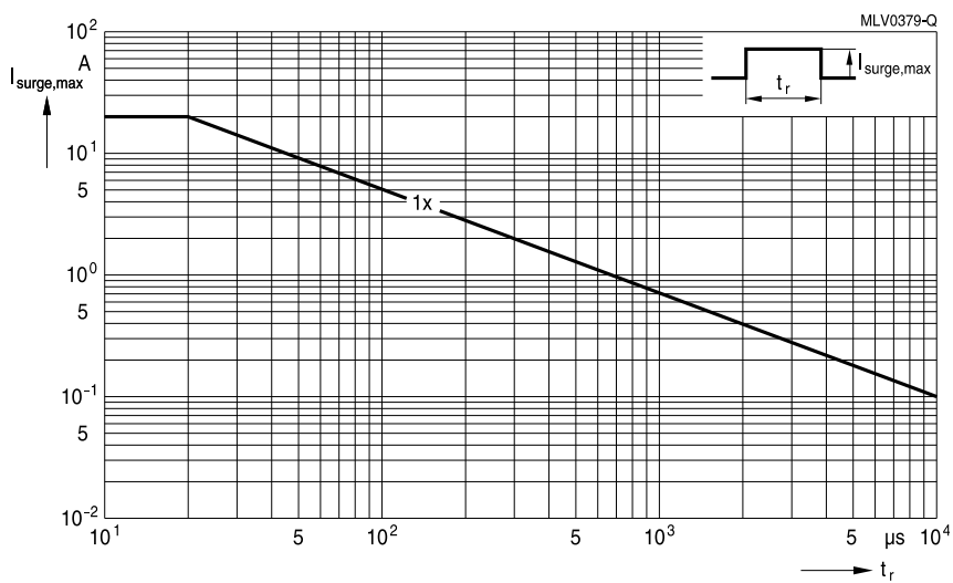
CT0402M4G ... S17AG
