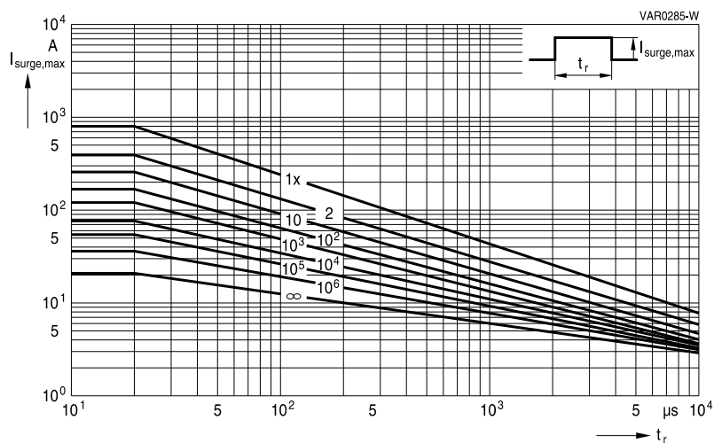
CN1812L8G ... K30G
