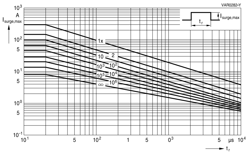
CT1210M6G
