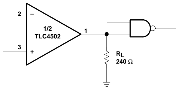
Figure 42. TTL-Driver Circuit
