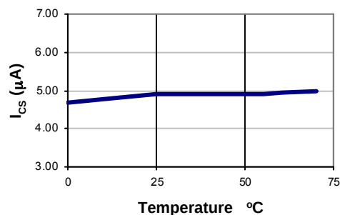
Figure 14: I_{CS} versus Temperature. Condition: V_{IN} = 3.0V
