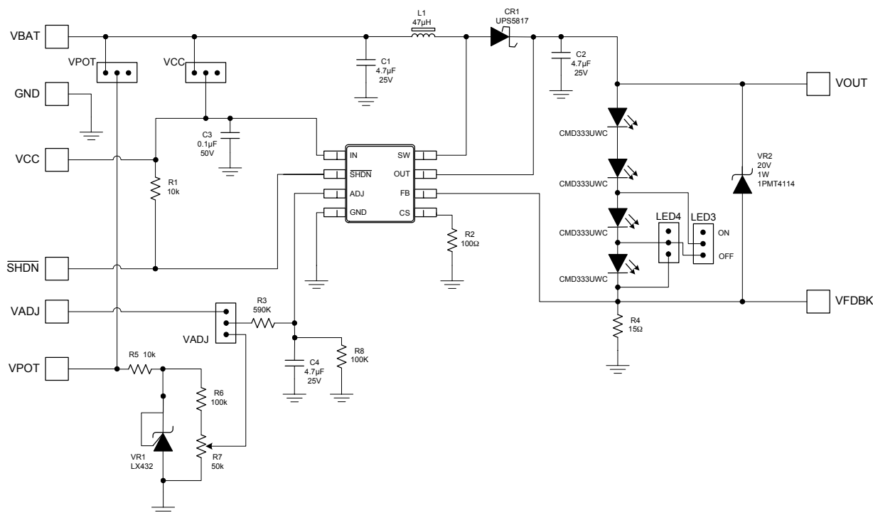
Figure 4 – LX1993 Boost Evaluation Board Schematic
