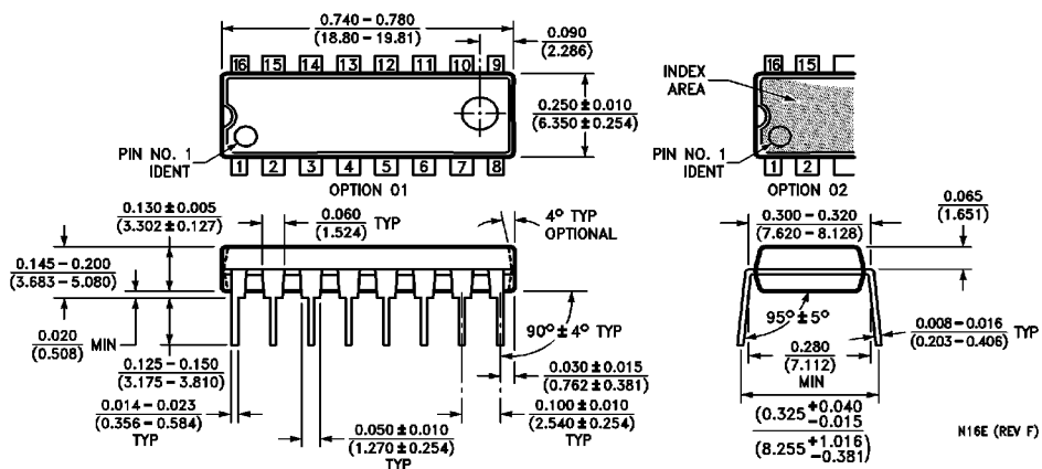
16-Lead Molded Dual-In-Line Package (N) Order Number DM74157N NS Package Number N16E
