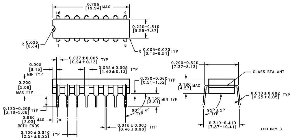
16-Lead Ceramic Dual-In-Line Package (J) Order Number 54157W or DM54157J NS Package Number J16A
