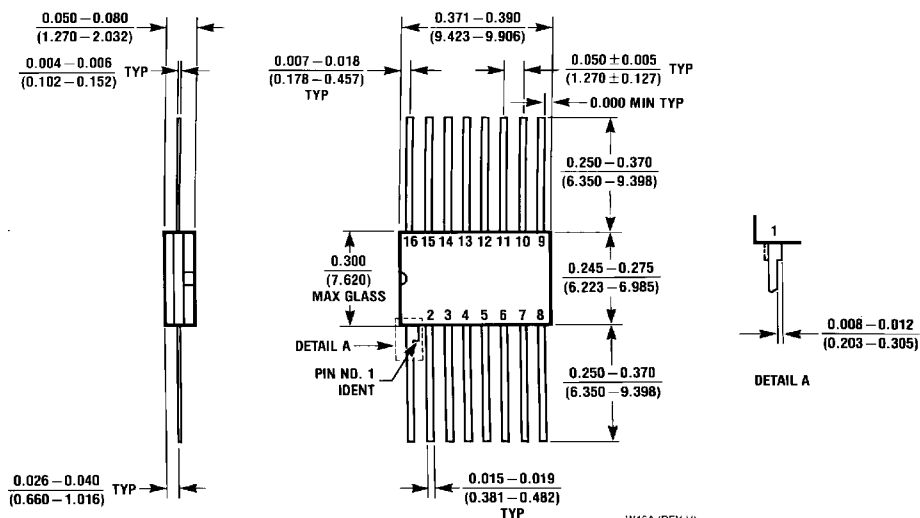
16-Lead Ceramic Flat Package (W) Order Number 54157FMBQ or DM54157W NS Package Number W16A
