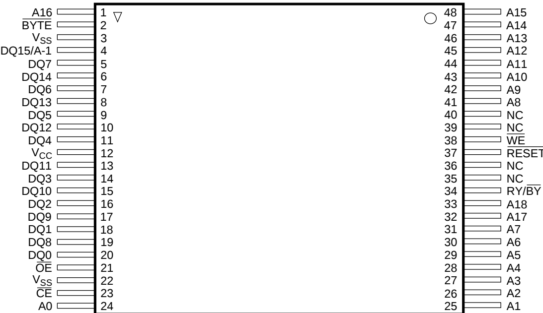
Reverse TSOP
