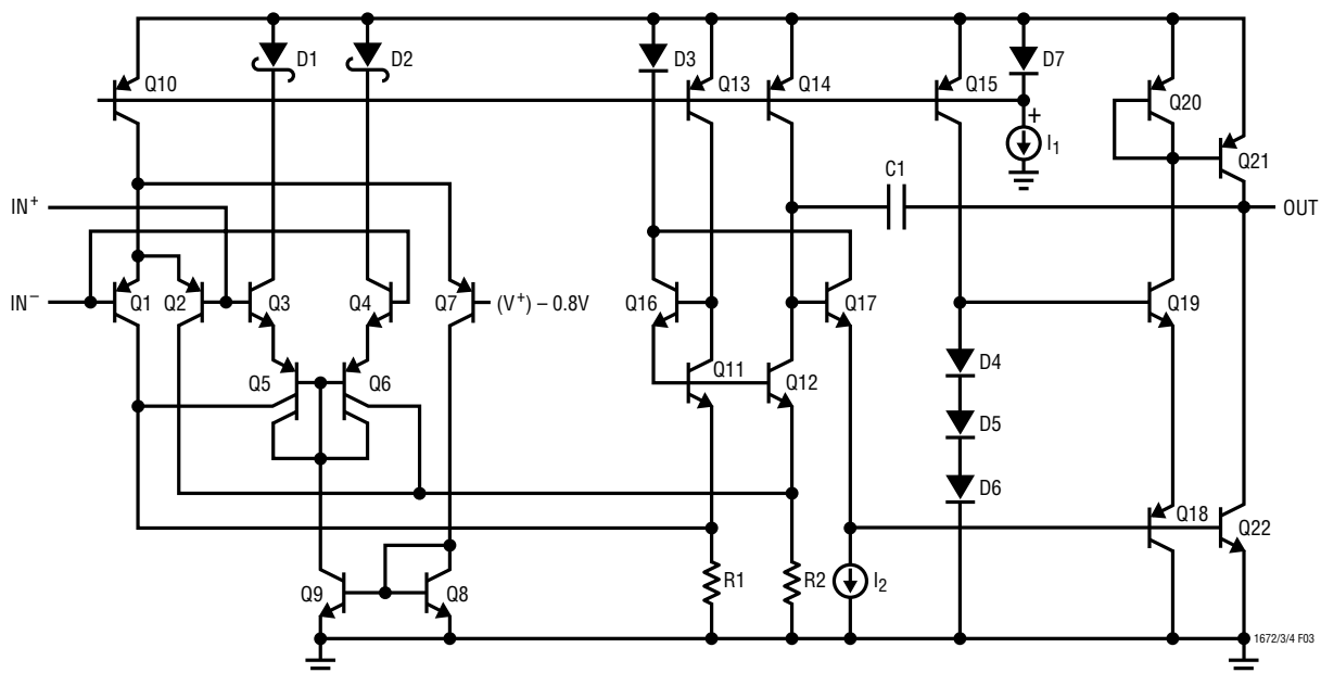
Figure 3. Simplified Schematic
