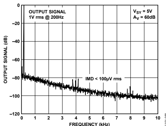
Figure 58. Spectral Analysis of AD8552 in High Gain with a 1 mV Input Signal
