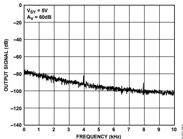
Figure 57. Spectral Analysis of AD855x Output with +60 dB Gain
