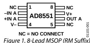
Figure 1. 8-Lead MSOP (RM Suffix)
