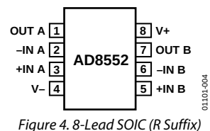
Figure 4. 8-Lead SOIC (R Suffix)
