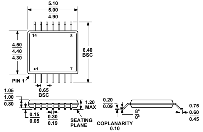
Figure 74. 14-Lead Thin Shrink Small Outline Package [TSSOP] (RU-14)
