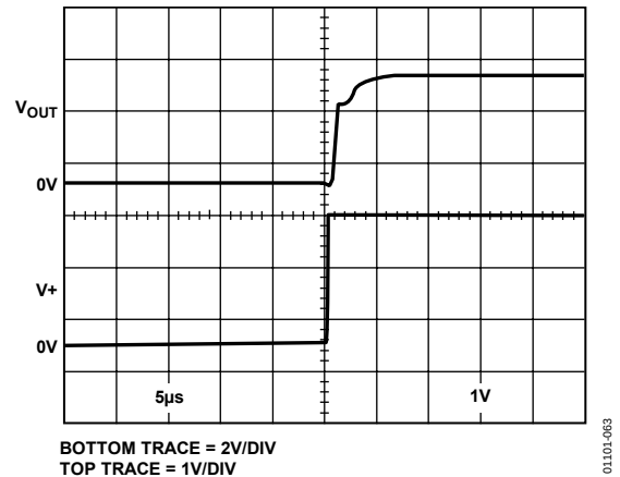
Figure 63. AD855x Output Behavior on Power-Up
